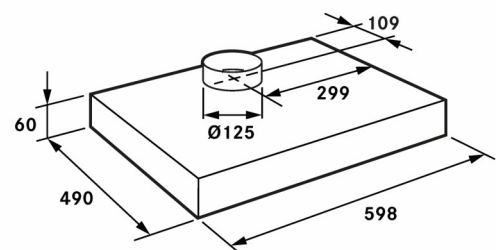
Central Plan 252
